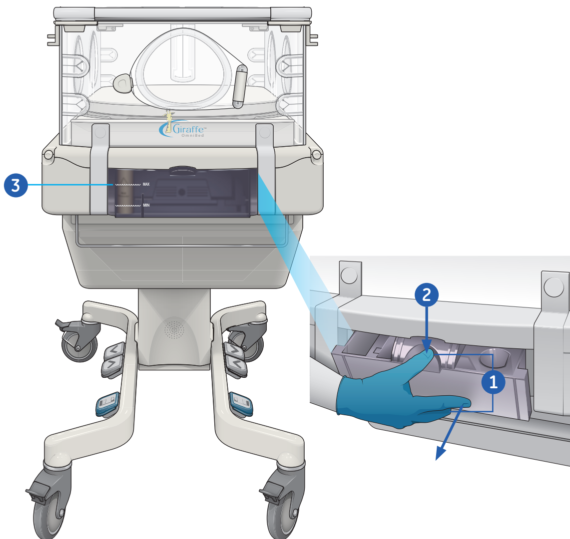
Figure 6.16 Water Reservoir Tilted for Filling
