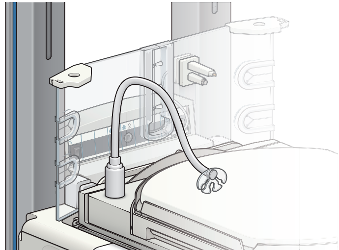
Figure 2.10 Mounting the tubing management arm
