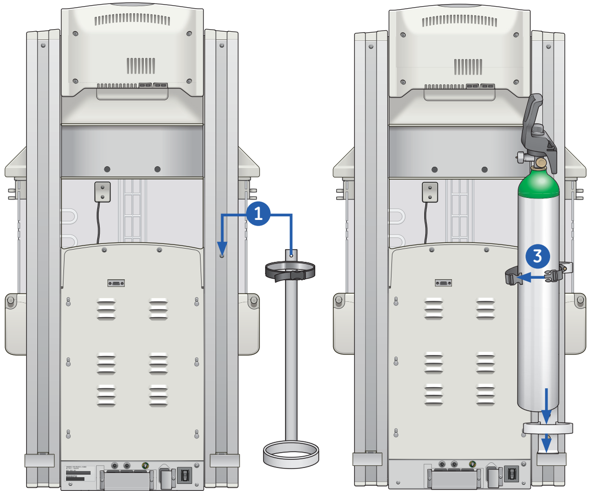
Figure 2.9 Mounting the gas cylinder holder
