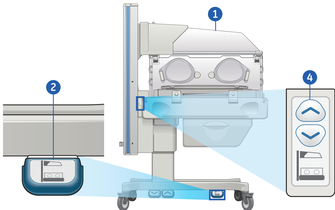
Figure 6.15 Raising and lowering the canopy
