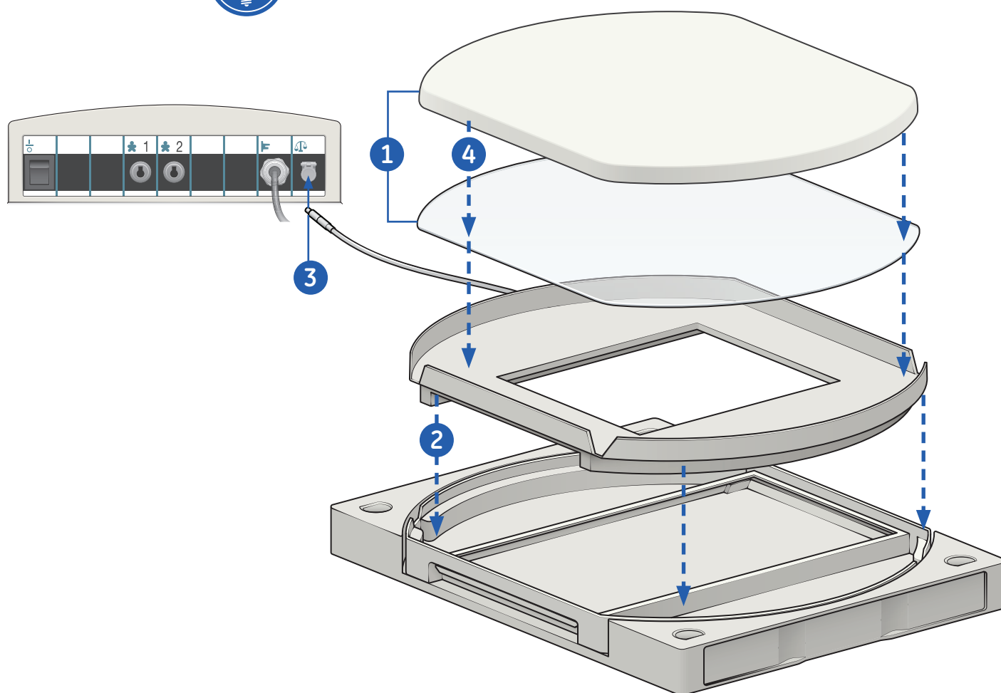
Figure 2.7 Installing the Scale
