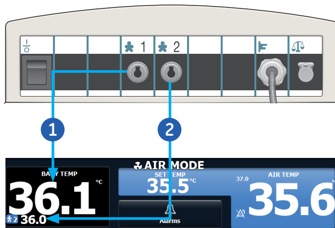
Figure 6.13 Two Probes in Use
